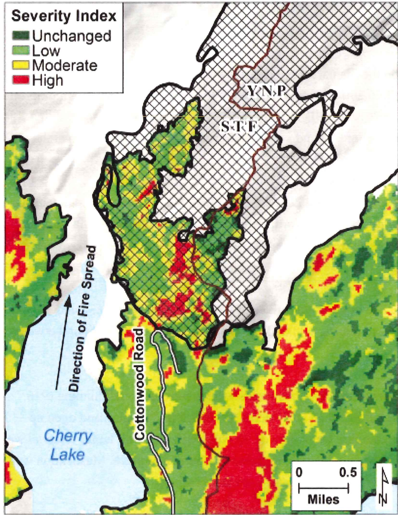
Figure 34. Kibbie Fire. Overview map of Kibbie Fire with initial fire severity.
